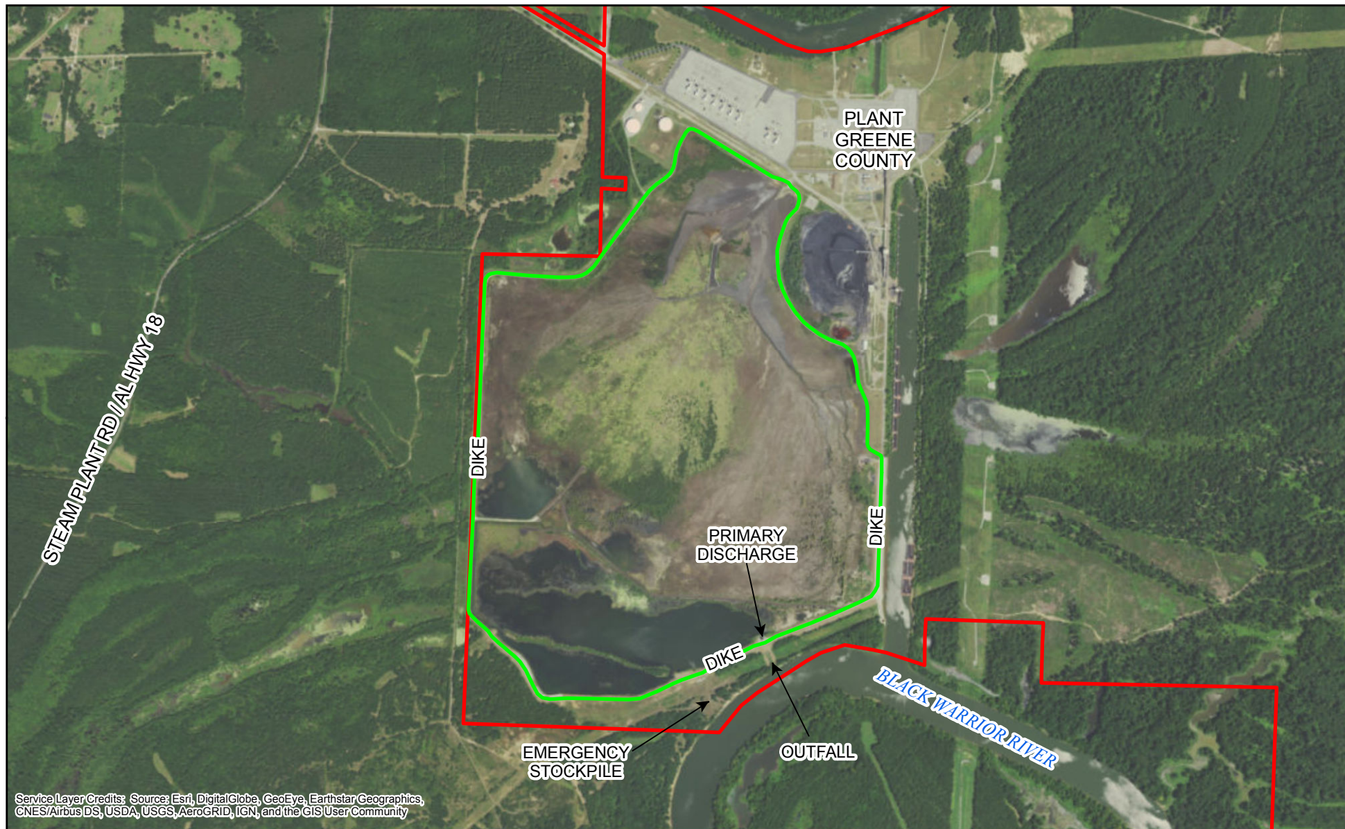
FIGURE 2 ASH POND OVERVIEW PLANT GREENE COUNTY GREENE COUNTY, ALABAMA
