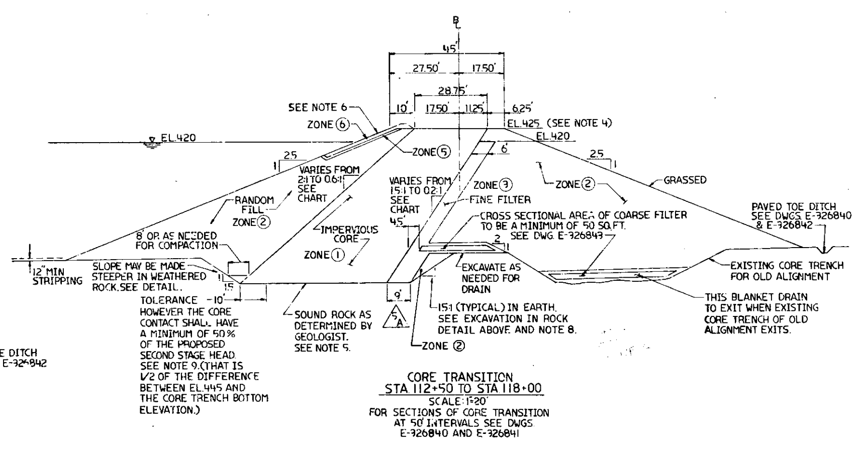
CORE SLOPES DURING TRANSITION STA 112+50 TO STA 118+00
