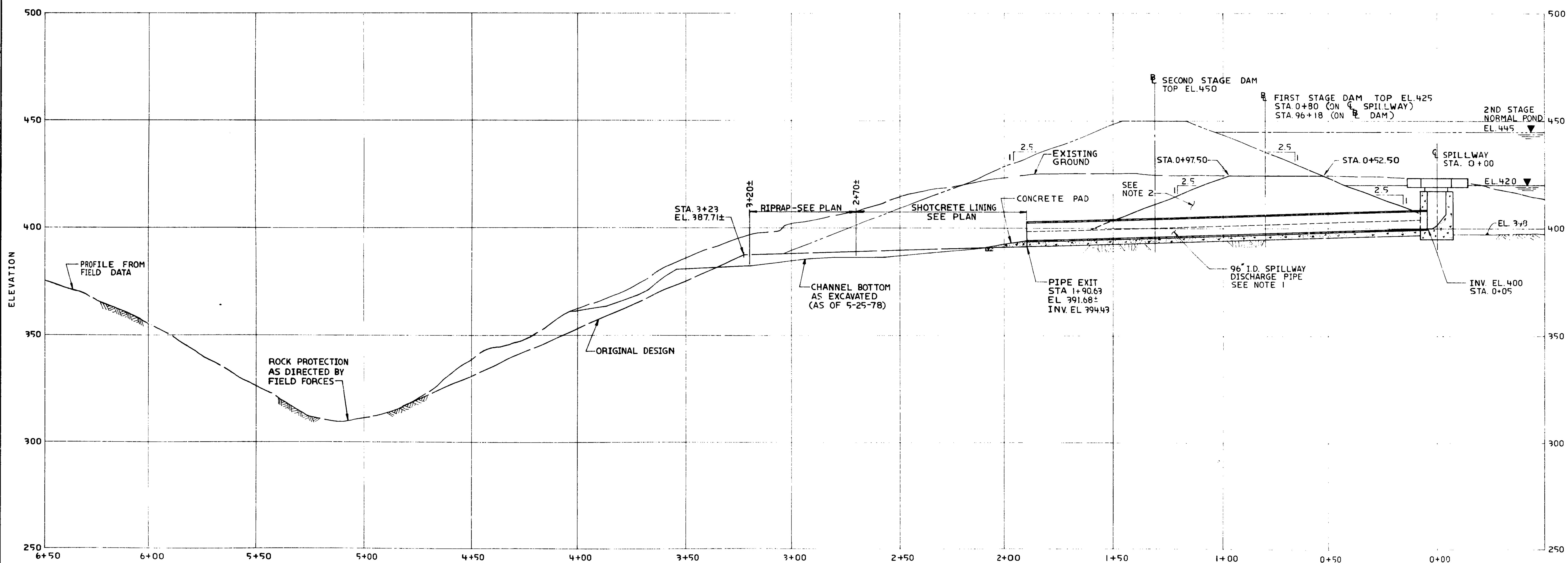
PROFILE ALONG C OF CHANNEL SCALE: 1"=20'
